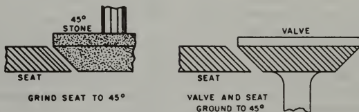
FIGURE 10-10. Fitting of the valve and seat.
